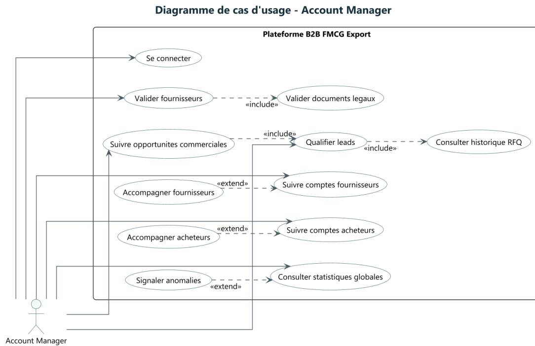
FIGURE 7 – Cas d'usage - account manager
